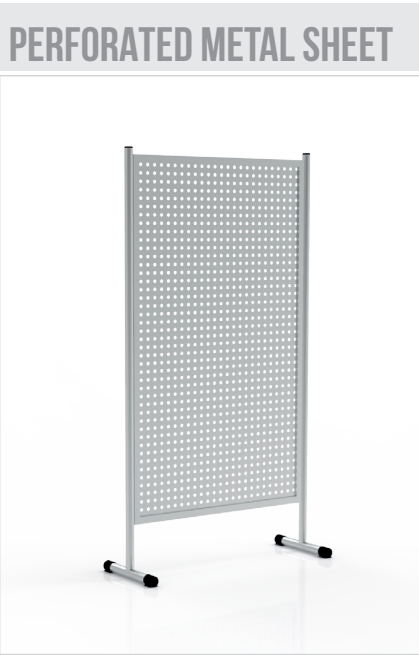
■ PERFORATED METAL SHEET ■ MOD. 7912AF15N DIMENSIONS: 110x70x155h. ■ MOD. 7912AF20N DIMENSIONS: 110x70x200h.
