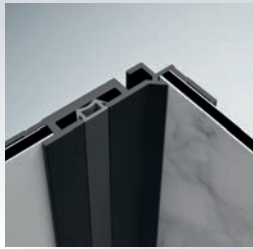
Montage met aluminium profielen Installation with aluminum profiles
